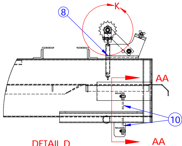
DETAIL D SCALE 1 : 12
