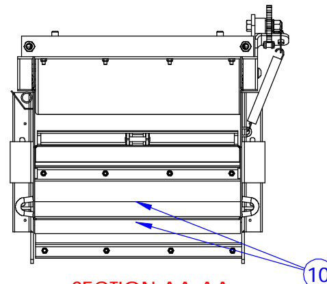
SECTION AA-AA SCALE 1 : 12
